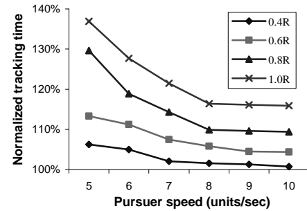
Figure 23: Normalized tracking time with different localization errors varying pursuer speed. Terrain size 1000 \times 1000 units, Radio range = 40units, density = 8 nodes per radio circle. Evader speed = 5 units /second
